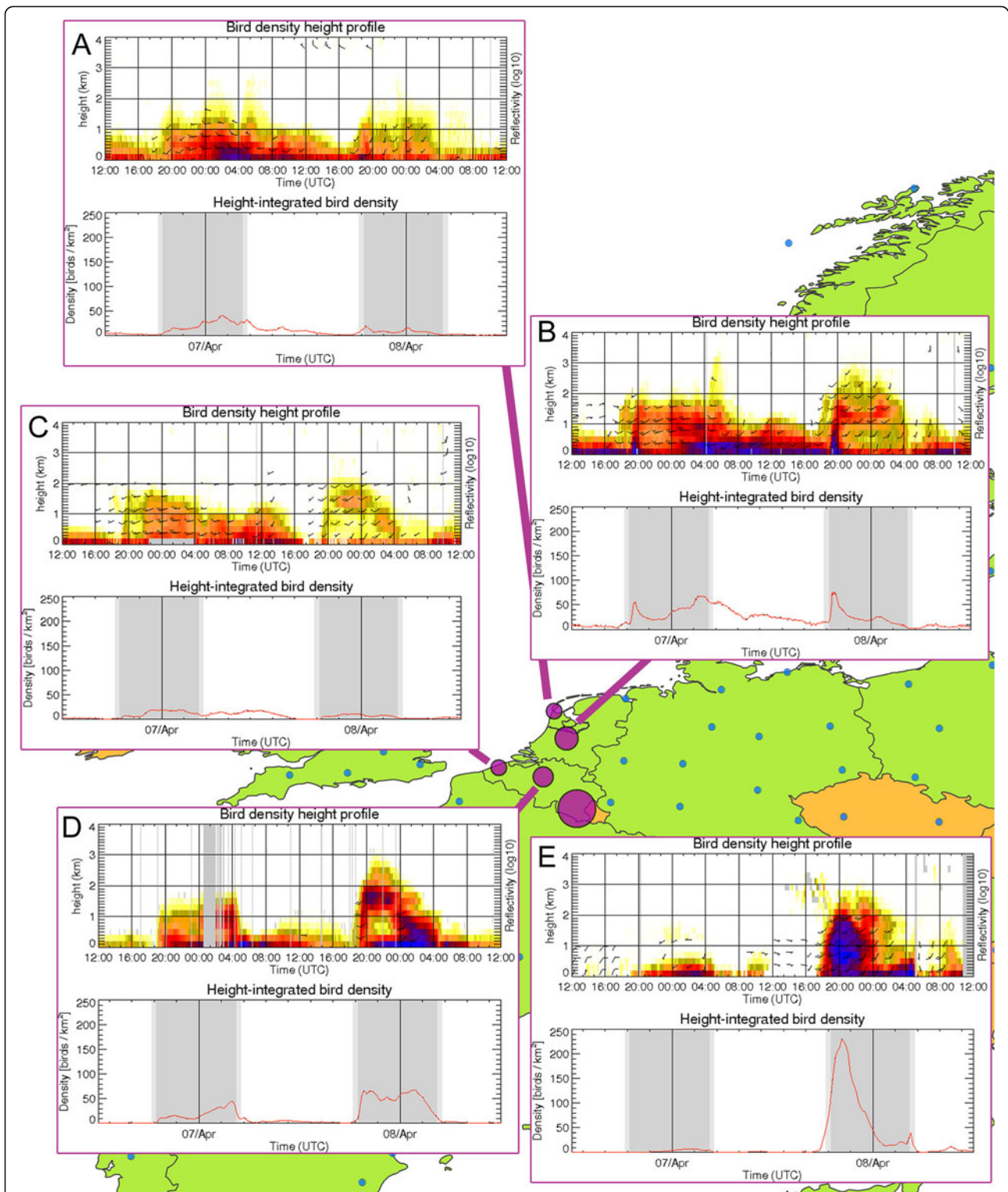
Figure 2 Mass bird migration observed on five operational weather radars. Nocturnal bird migration measured by two operational weather radars in the Netherlands ( A . Den Helder and B . De Bilt) and three operational weather radars in Belgium ( C . Jabbeke, D . Zaventem and E . Wideumont) on 7 and 8 April 2013 (for locations see purple circles on map, blue circles indicate other weather radars in the vicinity). The size of the purple circles represent the height-integrated bird density (birds/km 3 ) on 8 April 2013 at peak migration. Colours in upper graphs of each subplot indicate bird density (number of birds/km 3 ) with the wind bars indicating the birds' ground speed and flight direction, lower graphs in each subplot indicate the height-integrated bird density (birds/km 3 ), grey areas in these graphs indicate periods between dusk and dawn.
